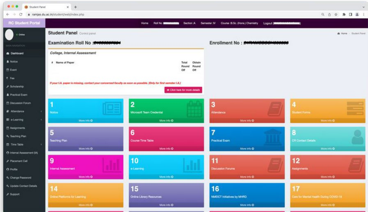
Student Dashboard
