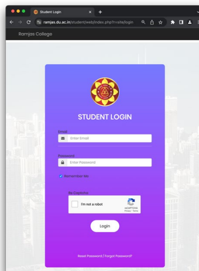
Login Screen
