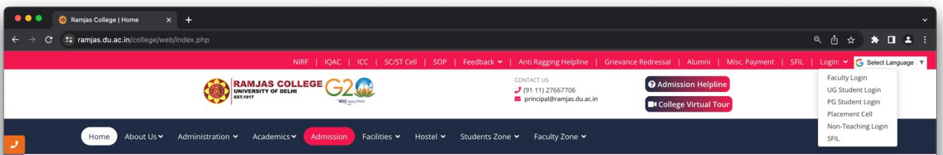
Website
