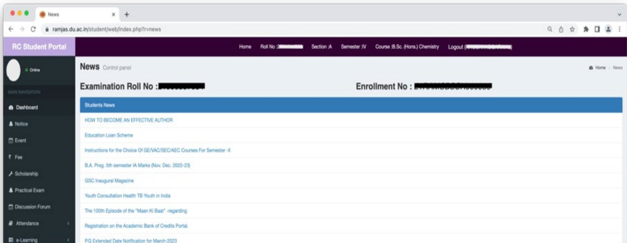
Student News
