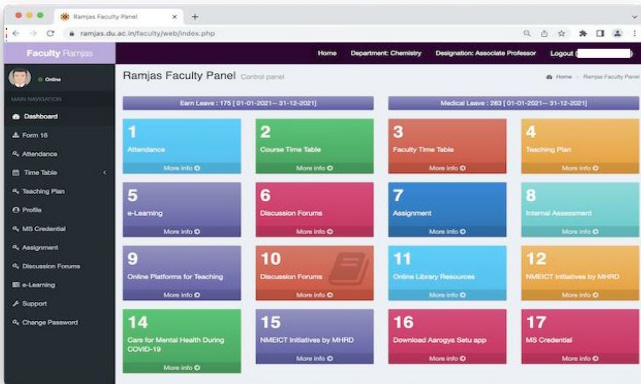
Faculty Dashboard
